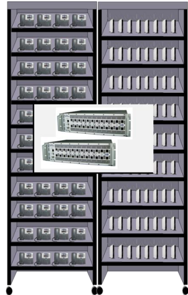
Traditional Rack of PD's vs 2x PSL-3424
